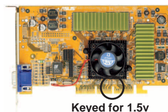
P4P800-E Accelerated Graphics Port (AGP)
